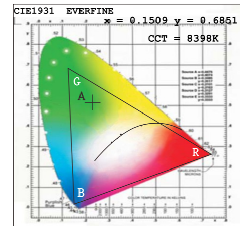
CIE1931 CHROMATICITY COORDINATES(Big Angle)
